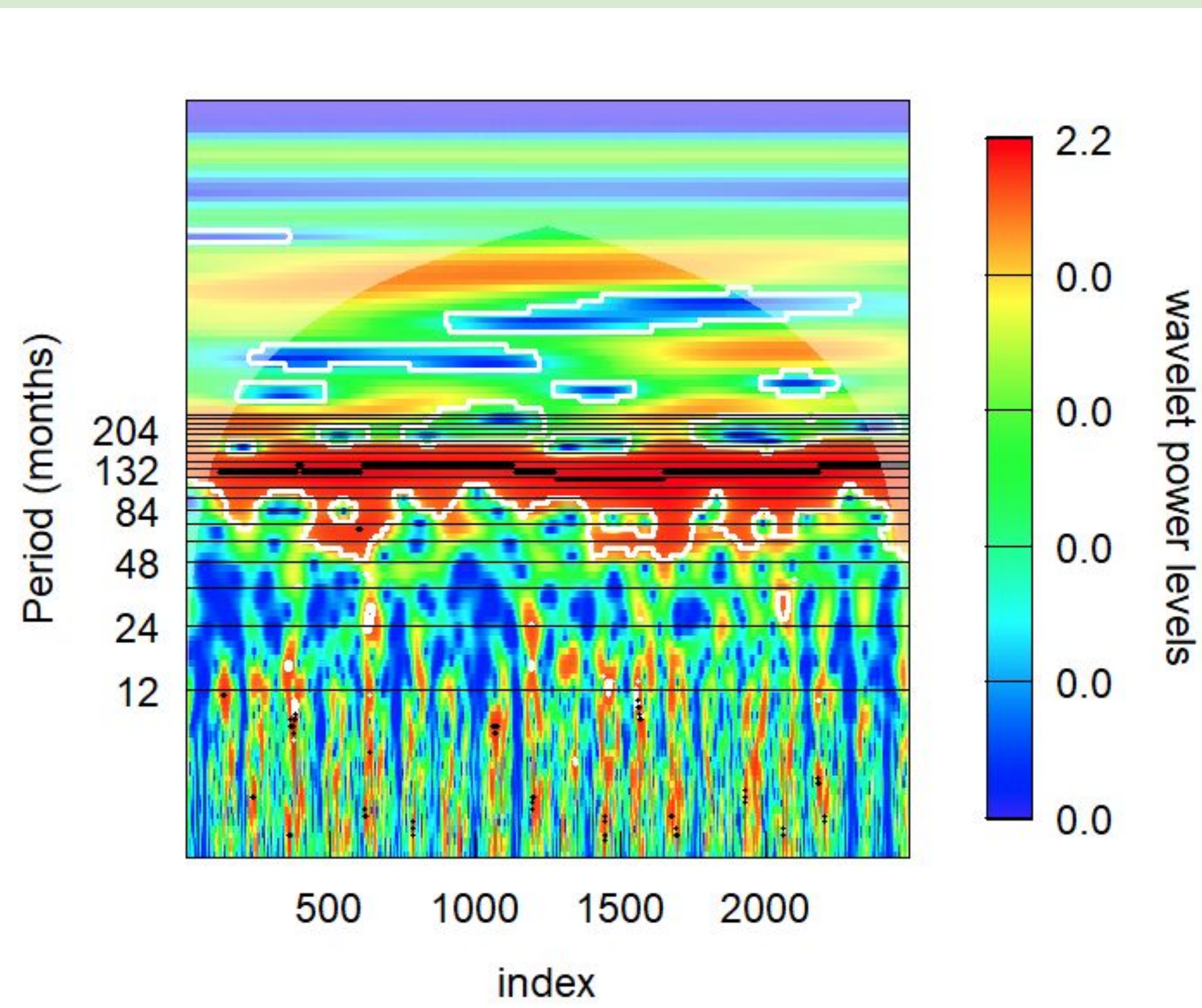
Figure 1: Wavelet showing the variable period of the raw sunspots number. Index value (x-axis) represents months during 1818-2025.
